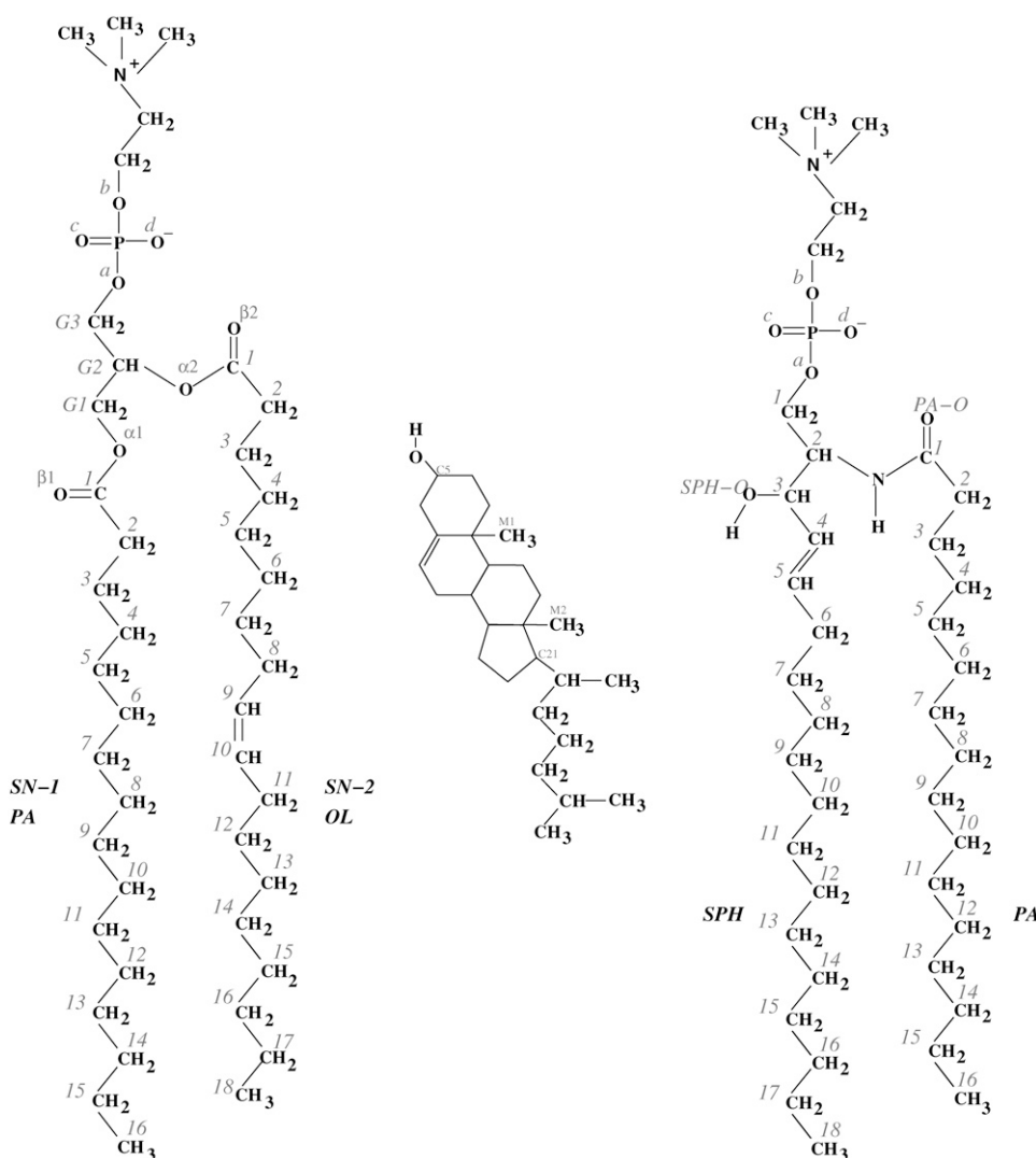
FIGURE 1 Structures of palmitoyl-oleoyl-phosphatidylcholine (POPC, left ), cholesterol (Chol, middle ), and palmitoyl-sphingomyelin (PSM, right ). Despite their broad structural similarities, POPC and PSM interact differently with Chol.
